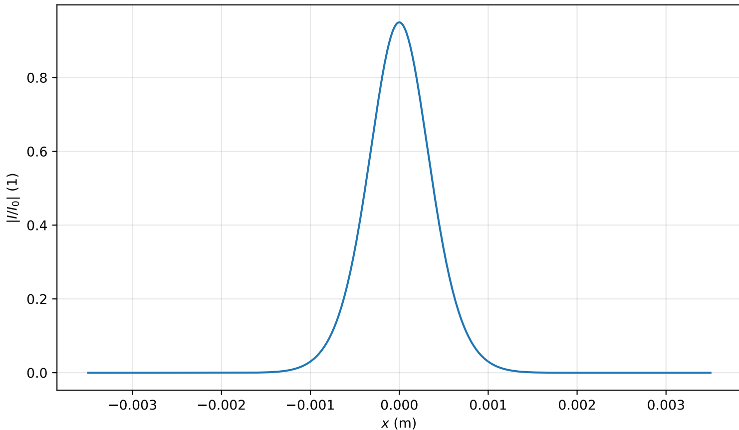
Intensity profile I(x, y = 0, z = 1.194m)/I_0 , \text{Pin}=0.4\text{Pcr} , artificial time
